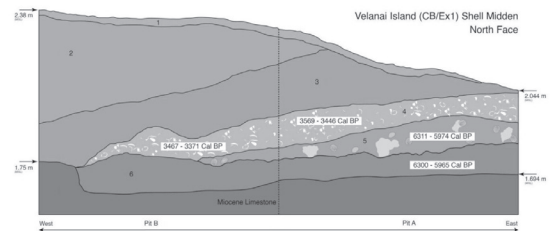
Figure 4. Stratigraphy of the profile excavated at CB/Ex1, north face.
