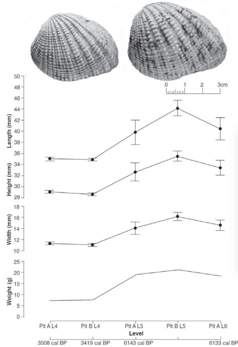
Figure 8. Average values of shell morphometrics of G. pectinatum from all levels of CB/Ex 01.
